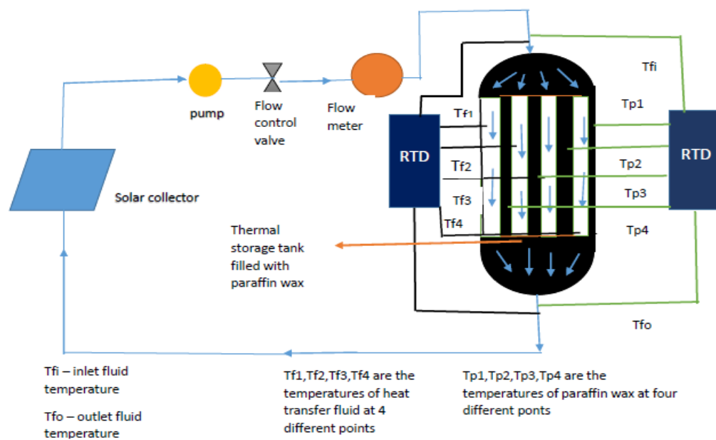
Fig.2. Shows the solar water heating system with PCM
