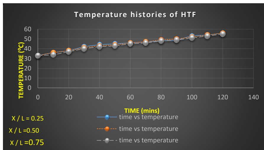
Fig. 11. Temperature histories of HTF at varying T_{fi} and mass flow rate 3litre / min
