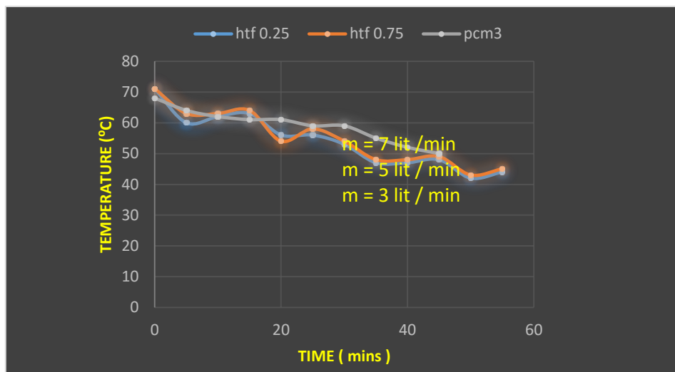
Fig .15 Effect of flow rate of the HTF, At varying T_{fi} , X/L = 0.50 , and mass flow rates
