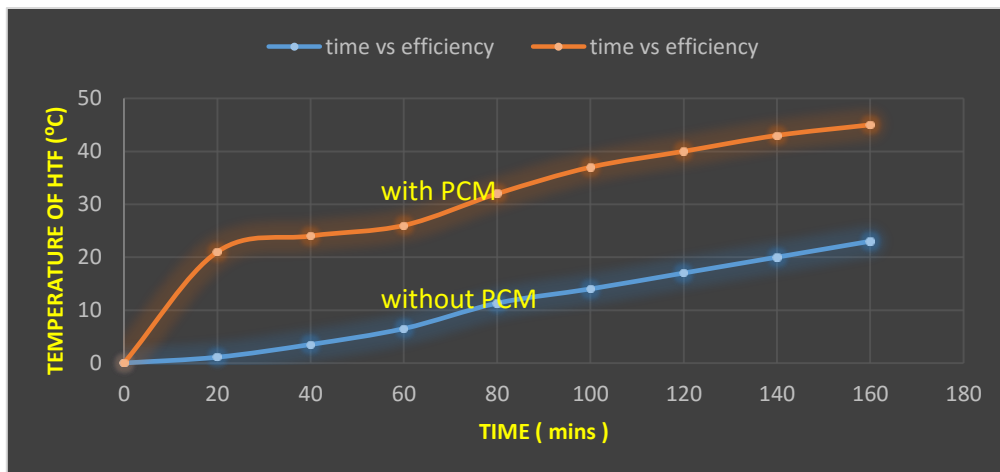
Fig. 17 shows the efficiency variation without using PCM and using PCM.
