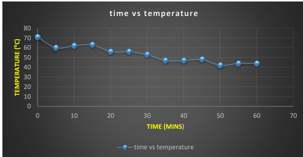
Fig.14. Effect of inlet fluid temperature on charging time.
