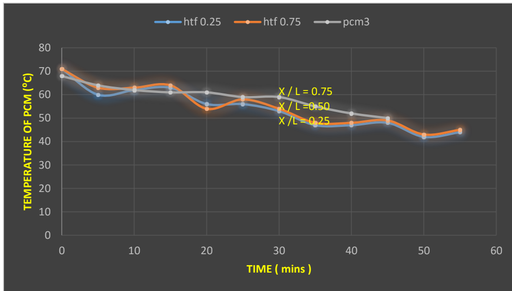
Fig. 18 Variation in the temperature of PCM during discharge process
