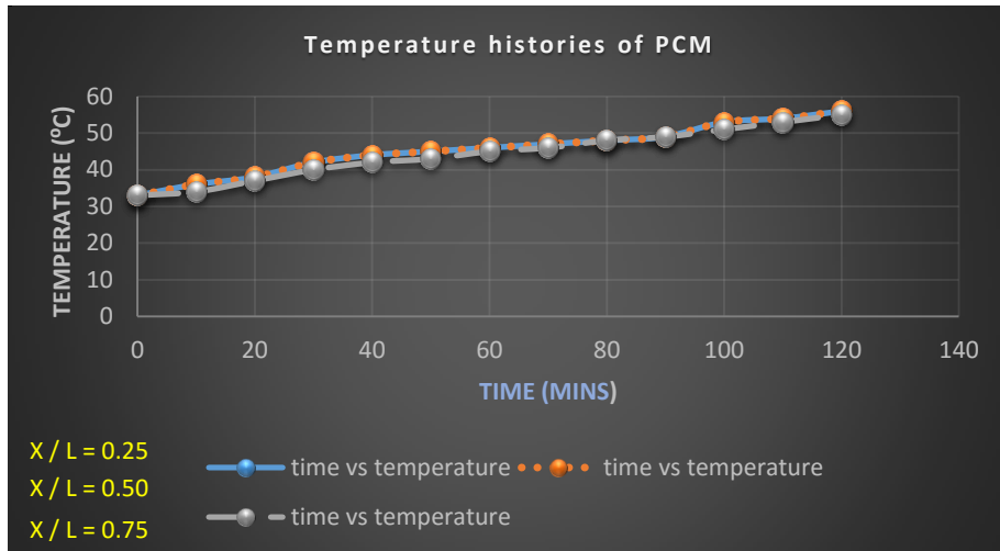
Fig. 12. Temperature histories of PCM
