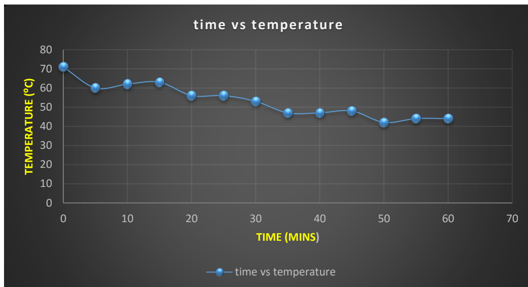
Fig.13 . Effect of inlet fluid temperature on charging time.
