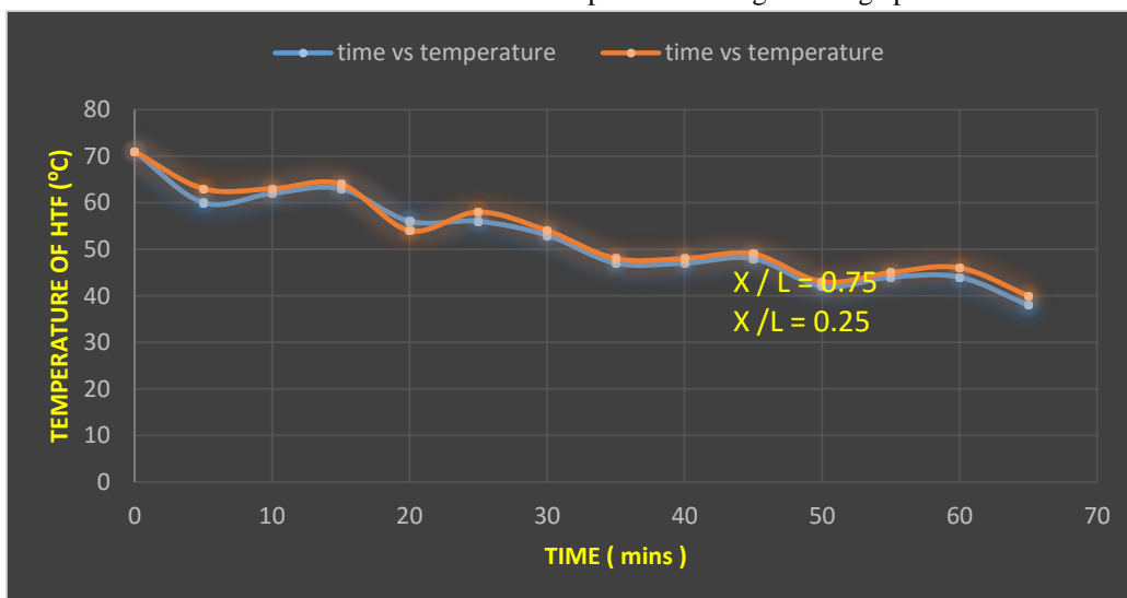
Fig.19. variation of HTF temperature during discharge process
