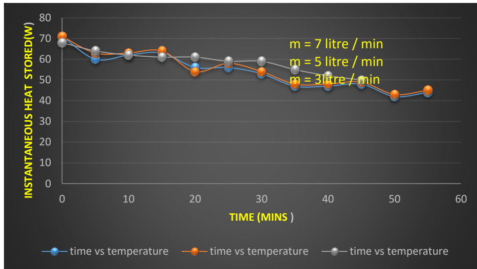
Fig.16 Instantaneous heat stored (in watts) for mass flow rates
